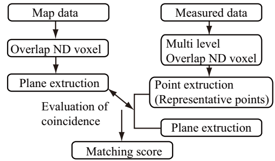
Fig. 10 Flow of likelihood calculation
