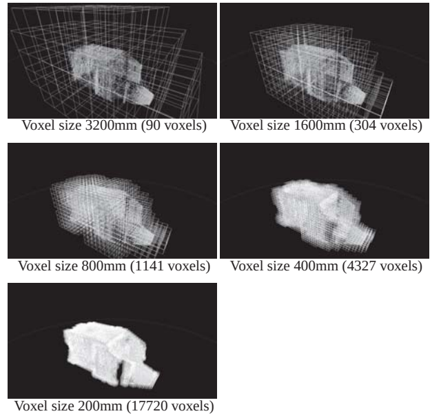
Fig. 9 Voxel resolution pyramid of eigen ellipses in elevator hall (indicated by circle in Fig.2)
