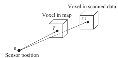
Fig. 20 Beam model for voxel representation
