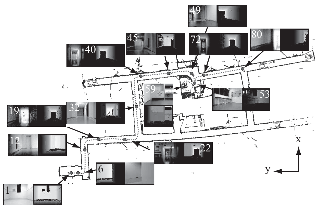
Fig. 12 Measuring positions for global positioning
