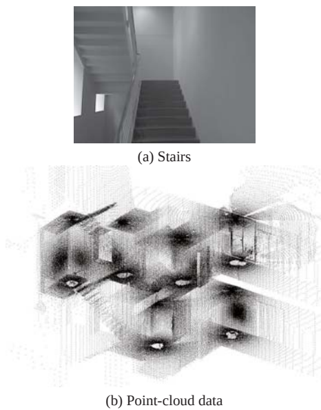
Fig. 17 Point-cloud data of stairs measured by a RGB-D camera
