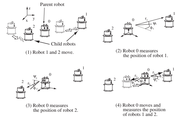
Fig. 6. Cooperative Positioning System (CPS)
