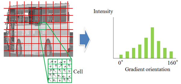
Fig. 5. Histogram of oriented gradients (HOG) feature for a reflectance image
